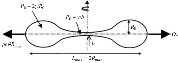
FIGURE 20. Sketch of an elongating two-lobed drop.
