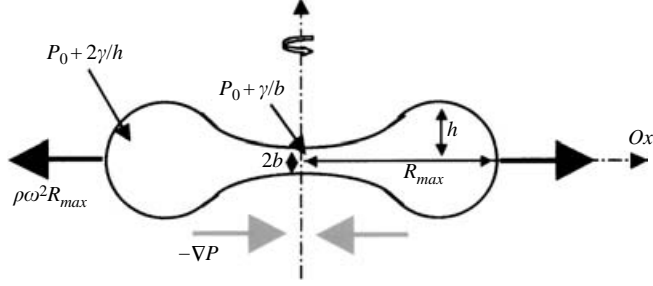
FIGURE 7. Forces acting on a two-lobed rotating drop.
