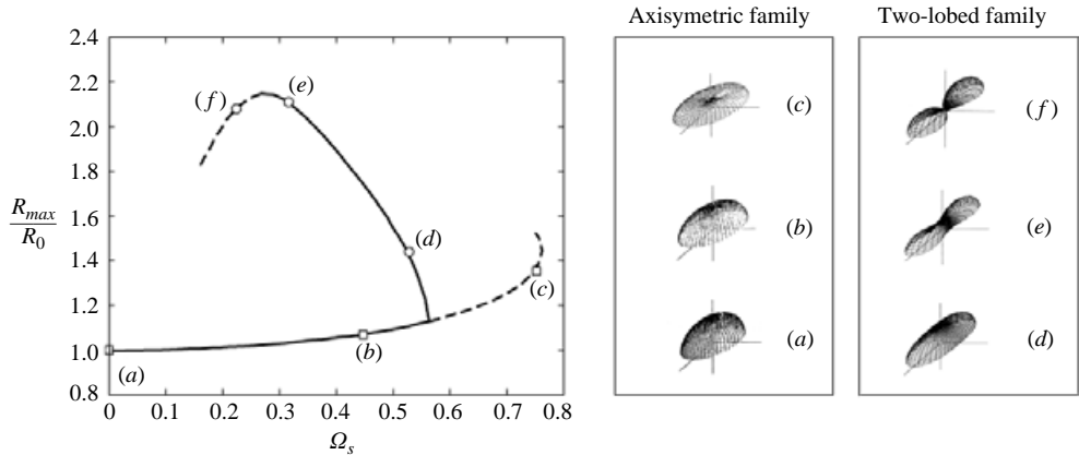
FIGURE 1. Phase diagram of axisymmetric ( a , b , c ) and two-lobed ( d , e , f ) isolated drops in rotation (Brown & Scriven 1980 a ). The maximum size of the centrifuged drop is normalized by its initial radius and plotted as a function of the angular speed of rotation \Omega_s , made dimensionless as defined in equation (1). The full lines indicate stable shapes. Six examples of shapes computed by Brown & Scriven are also displayed.
